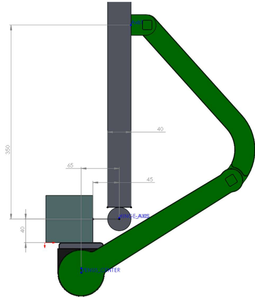
ADAPTERPLATE OFFSET
