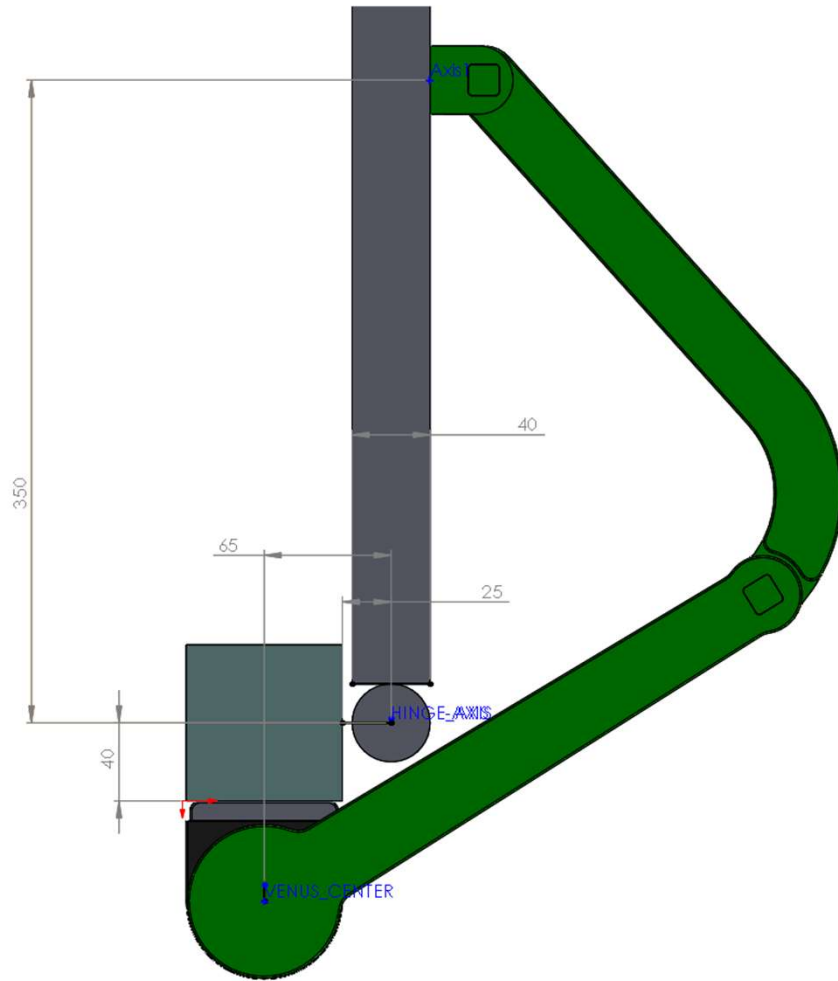
ADAPTERPLATE CENTERED
